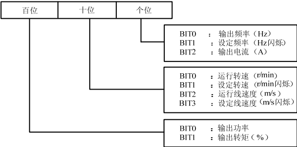
图6-71 LED 运行显示参数选择 1 设定
