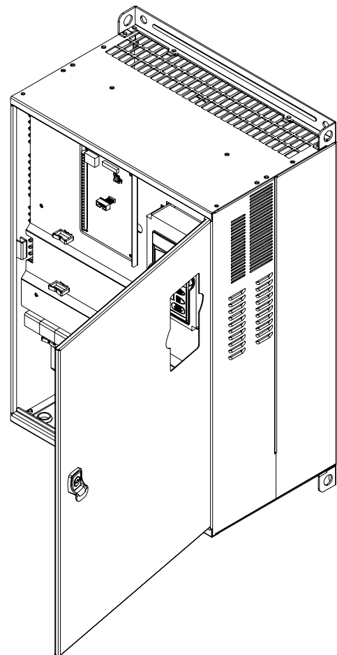
75-100HP/55-75kW(Frame F)
