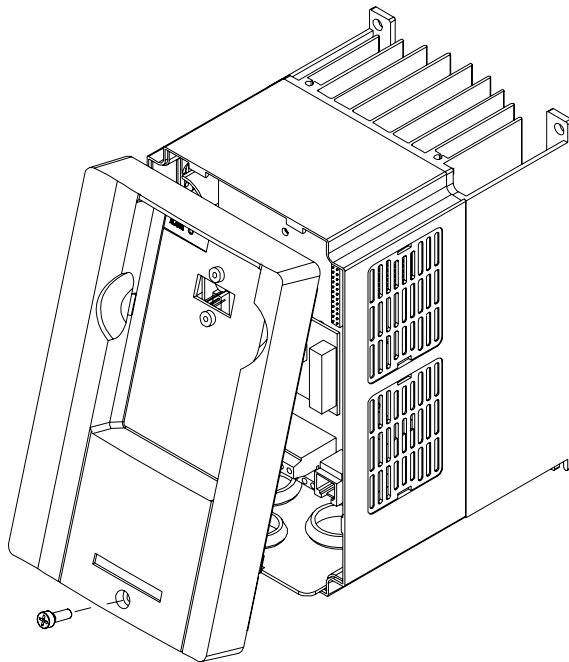
1-3HP/0.75-2.2kW(Frame A, A1, A2)
