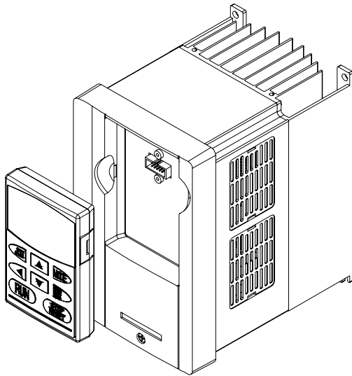
1-3HP/0.75-2.2kW(Frame A, A1, A2)
