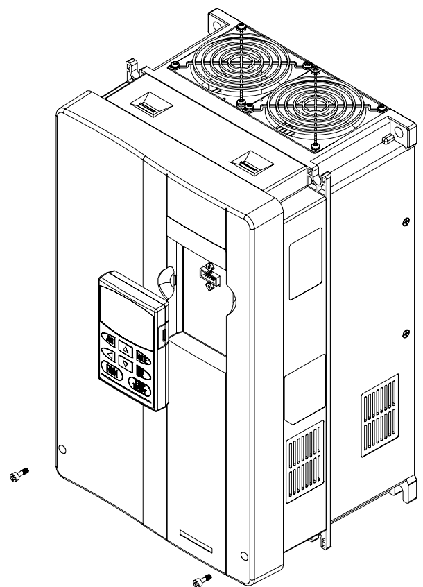
20-30HP/15-22kW(Frame D)
